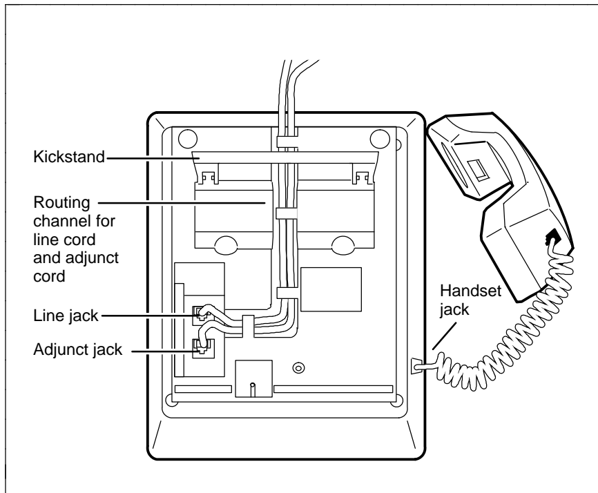
FIGURE 5 Line, Adjunct, and Handset Cord Routing for Desktop Installation
