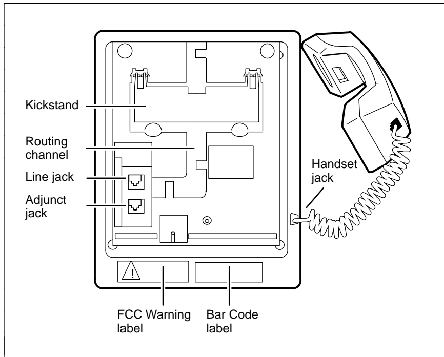
FIGURE 2 8510T Voice Terminal (Bottom View With Kickstand)
